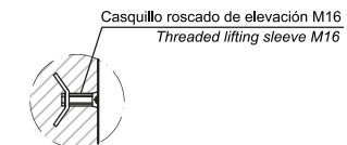
DETALLE M / DETAIL M
